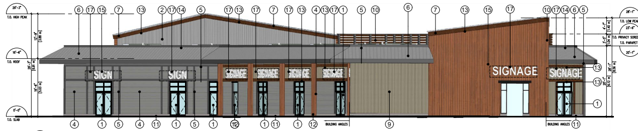
1 NORTH ELEVATION ASB 1/8"=1'-0"
