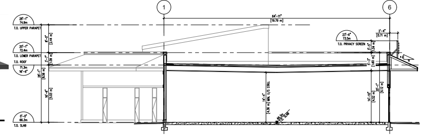
5 BUILDING SECTION ASB 1/8"=1'-0"
