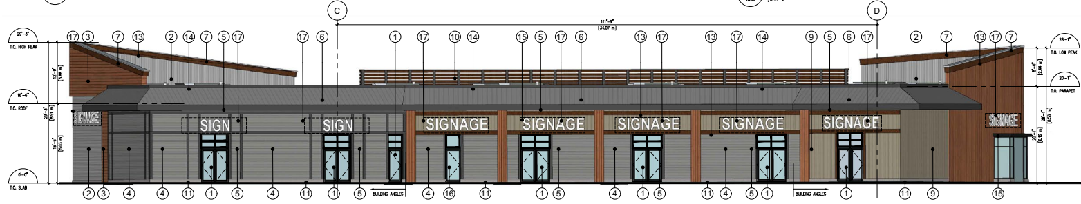
3 EAST ELEVATION ASB 1/8"=1'-0"
