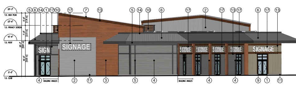
2 SOUTH ELEVATION ASB 1/8"=1'-0"
